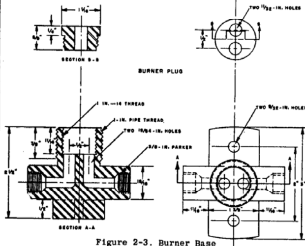
Figure 2-3. Burner Base
