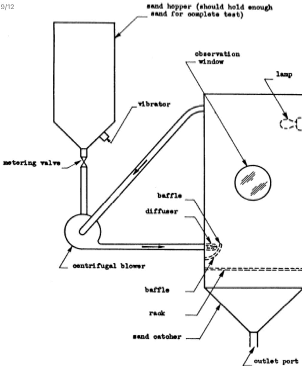
FIGURE 1 Schematic Sand Test Arrangement (Ref. Section 7.8)
