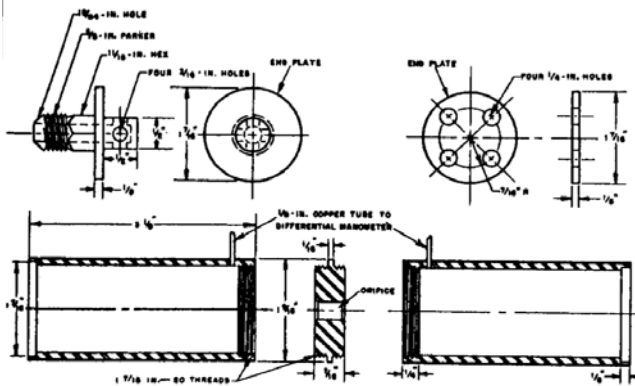
Figure 2-4. Orifice Chamber
