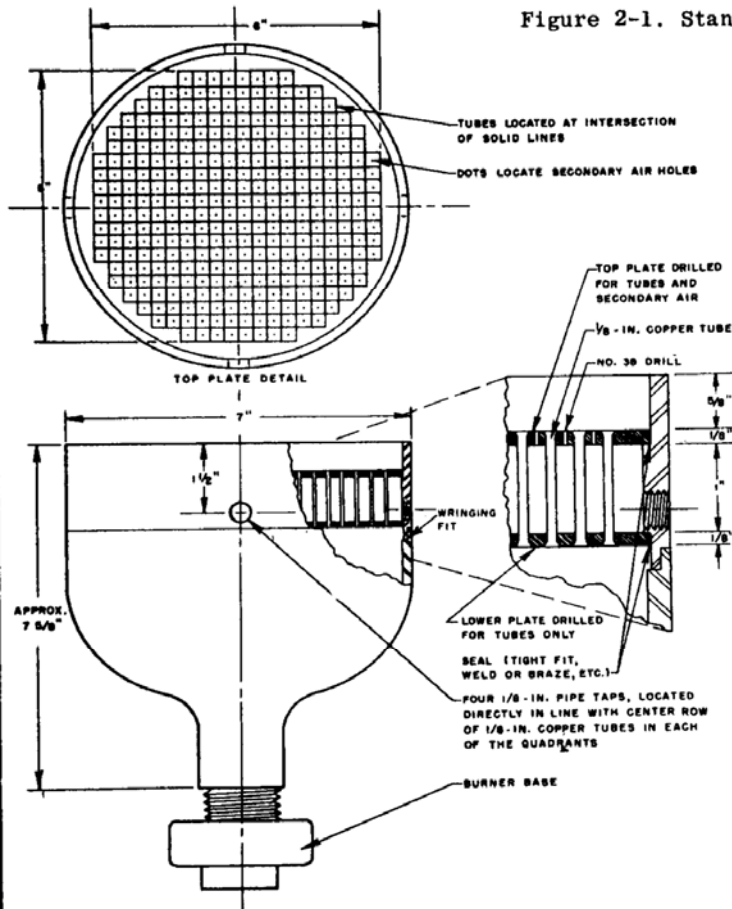
Figure 2-2. Standard Burner
